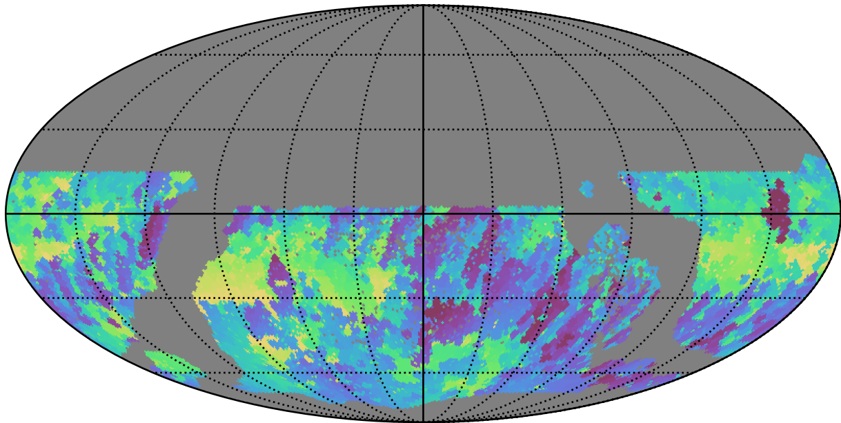
too_100_4v3.4_10yrs WFD r band: Min skyBrightness
