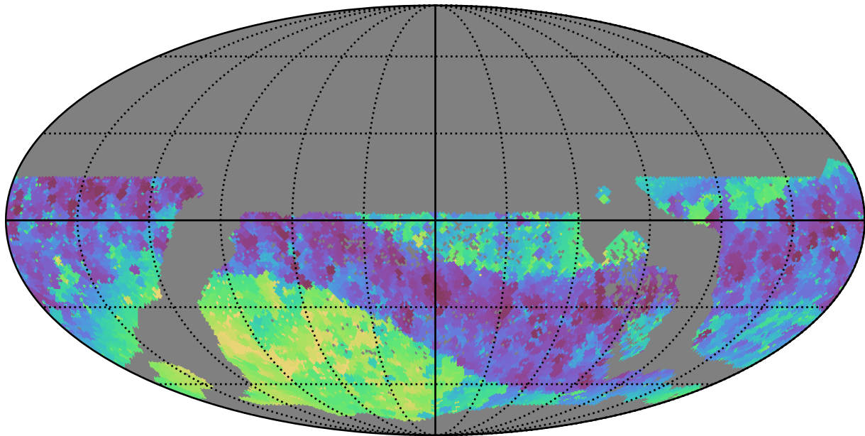
too_100_4v3.4_10yrs WFD i band: Min skyBrightness
