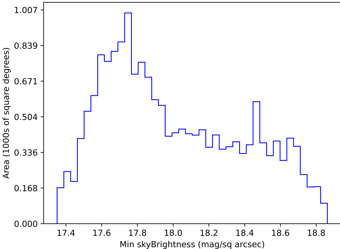
too_100_4v3.4_10yrs WFD i band: Min skyBrightness
