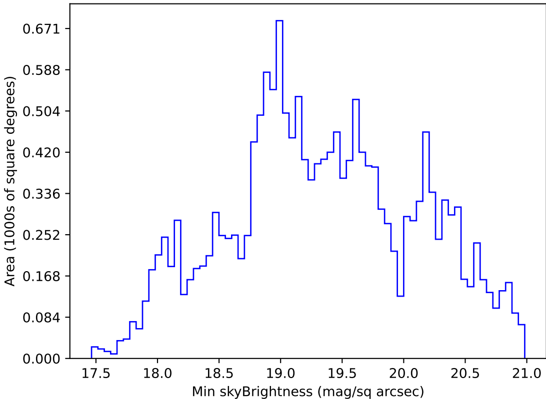
too_100_4v3.4_10yrs WFD g band: Min skyBrightness
