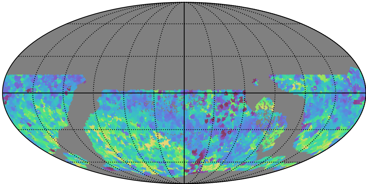
too_100_4v3.4_10yrs WFD all bands: Min skyBrightness
