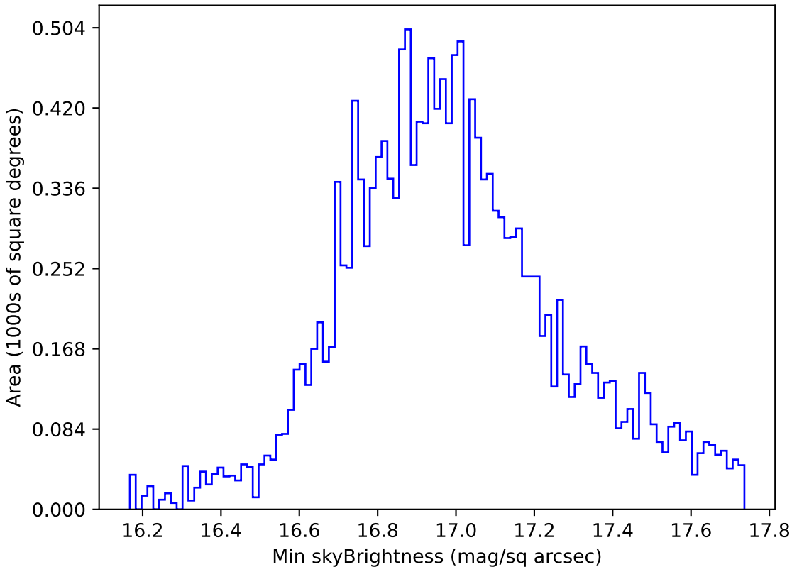
too_100_4v3.4_10yrs WFD all bands: Min skyBrightness
