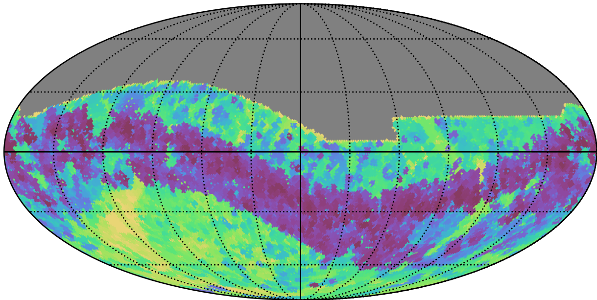
too_100_4v3.4_10yrs All sky z band: Min skyBrightness
