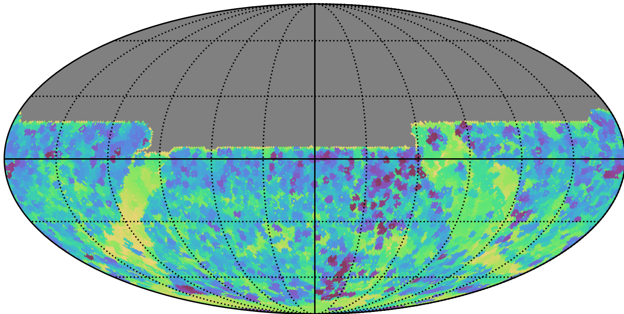
too_100_4v3.4_10yrs All sky y band: Min skyBrightness
