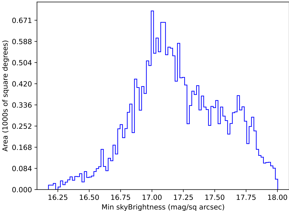
too_100_4v3.4_10yrs All sky y band: Min skyBrightness
