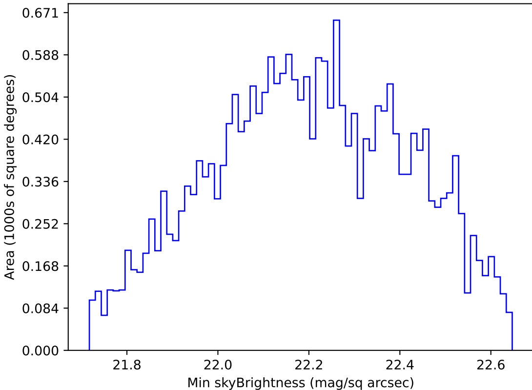
too_100_4v3.4_10yrs All sky u band: Min skyBrightness
