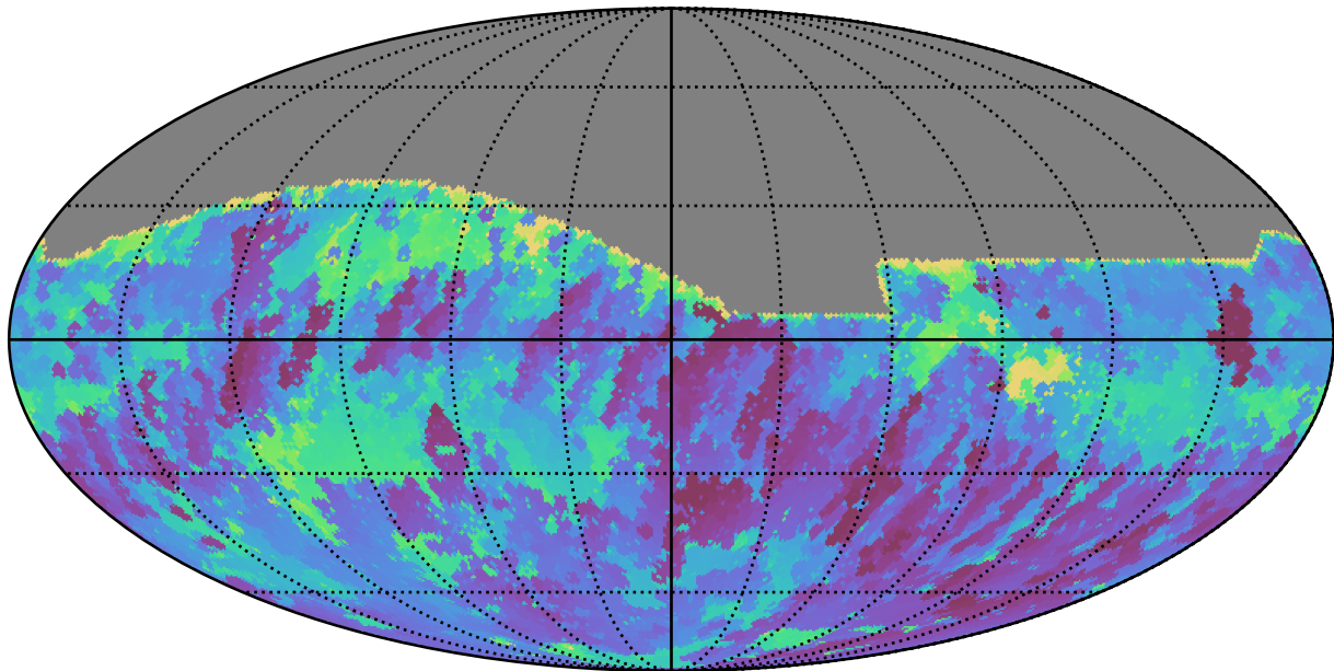
too_100_4v3.4_10yrs All sky r band: Min skyBrightness
