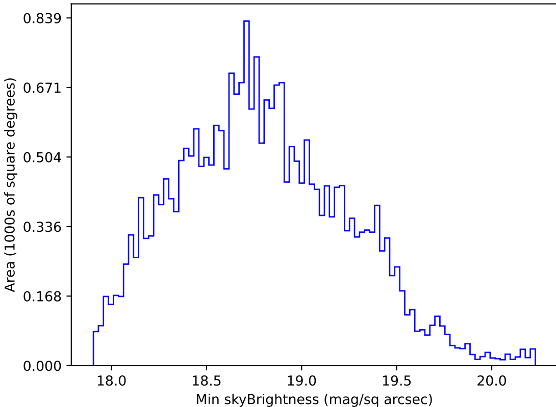
too_100_4v3.4_10yrs All sky r band: Min skyBrightness
