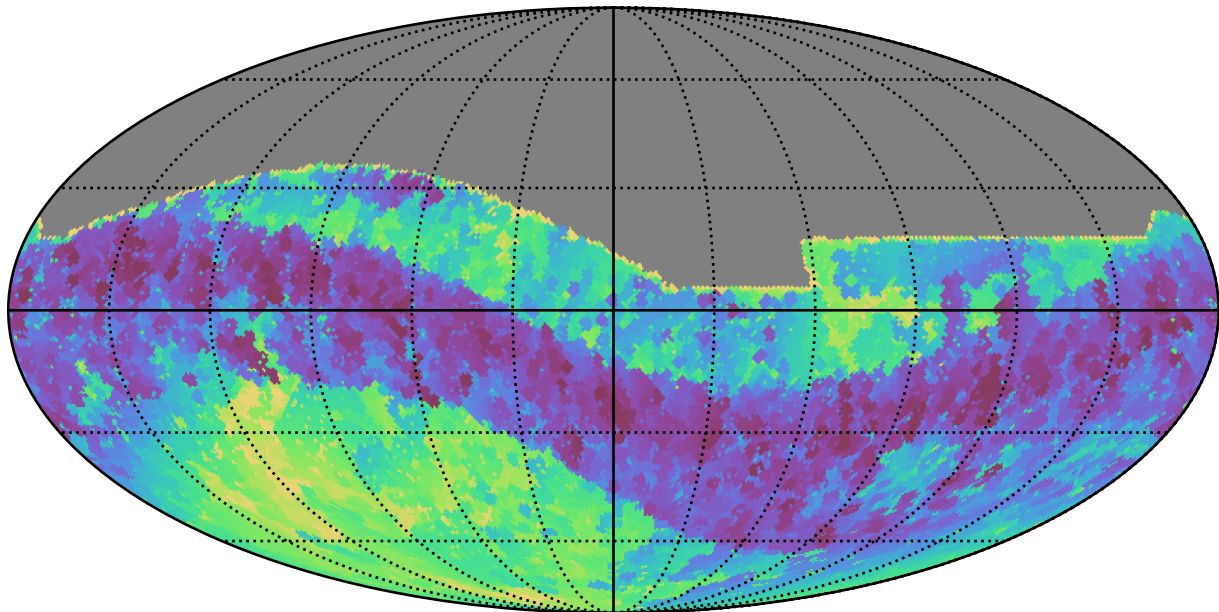
too_100_4v3.4_10yrs All sky i band: Min skyBrightness
