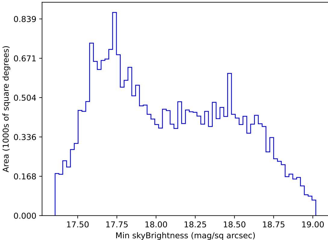
too_100_4v3.4_10yrs All sky i band: Min skyBrightness
