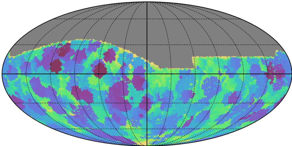
too_100_4v3.4_10yrs All sky g band: Min skyBrightness
