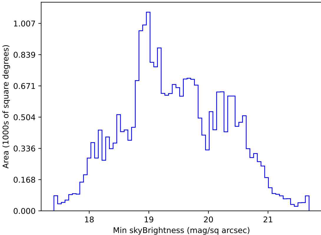
too_100_4v3.4_10yrs All sky g band: Min skyBrightness
