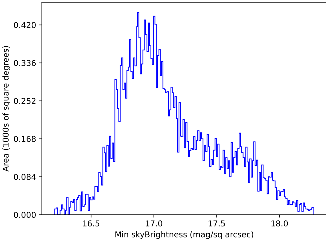
too_100_4v3.4_10yrs All sky all bands: Min skyBrightness
