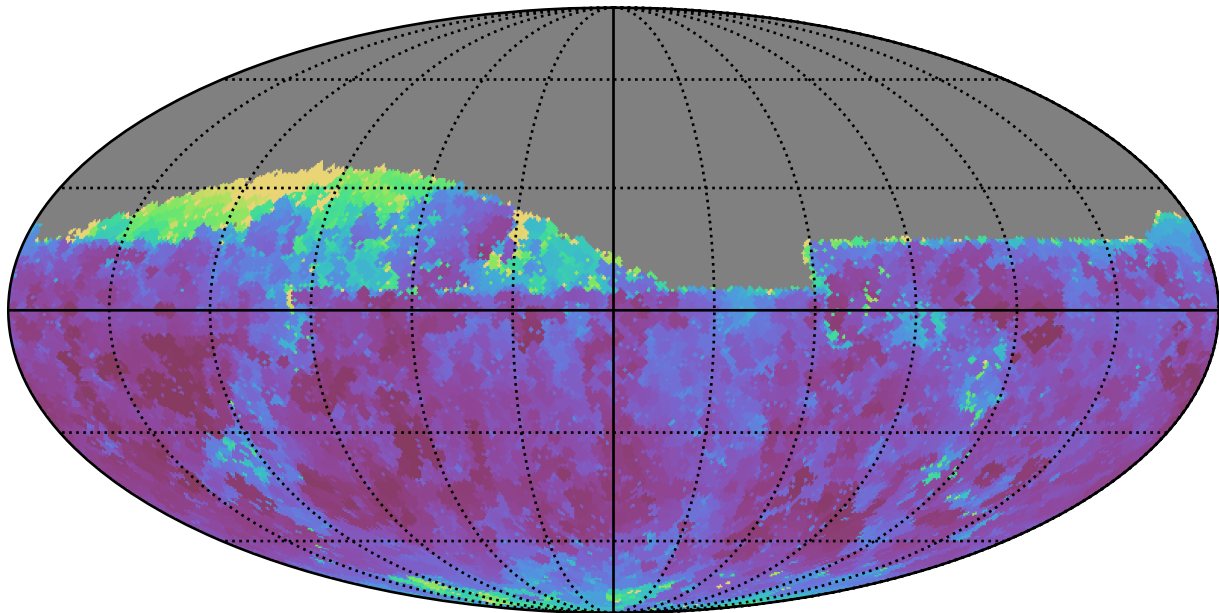
too_100_4v3.4_10yrs Yr 1 z band: Min seeingGeom
