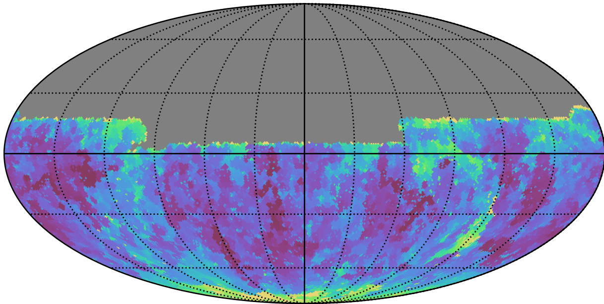
too_100_4v3.4_10yrs Yr 1 y band: Min seeingGeom
