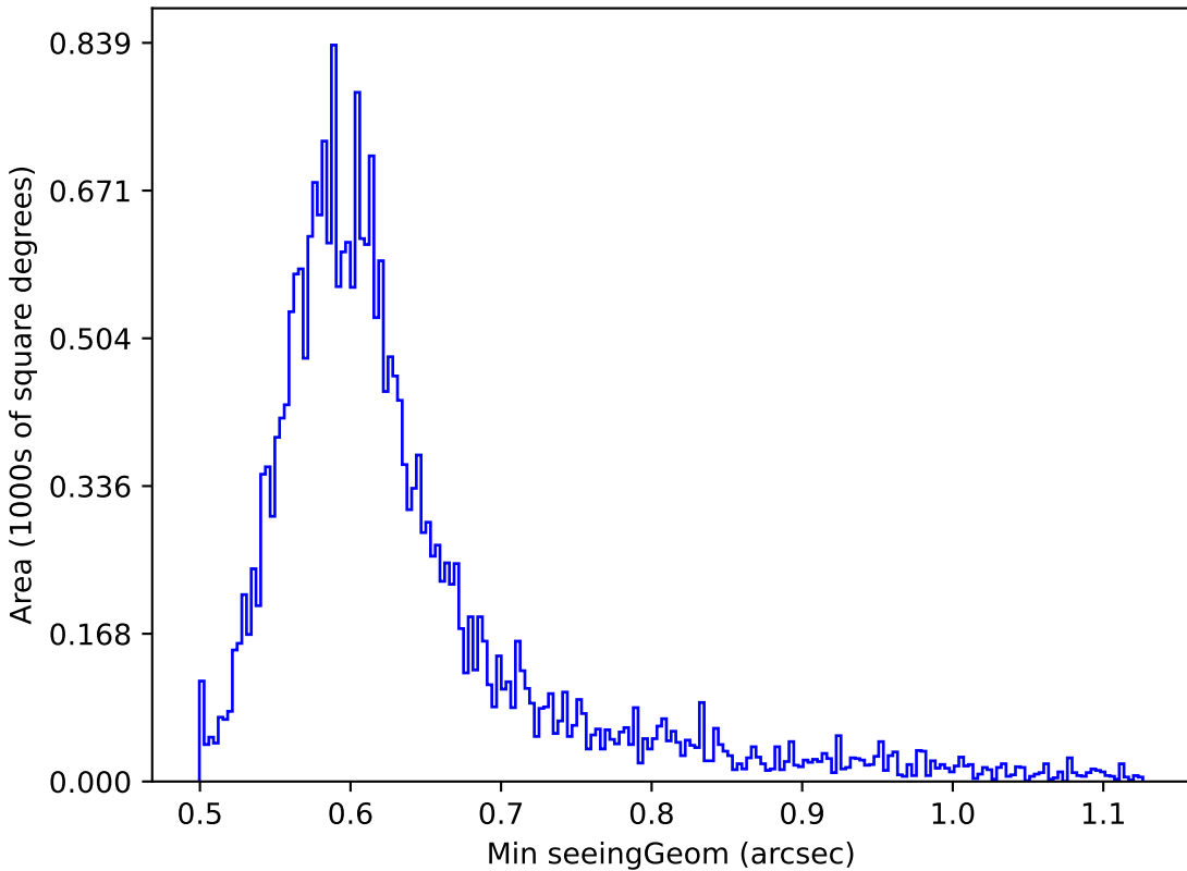
too_100_4v3.4_10yrs Yr 1 i band: Min seeingGeom
