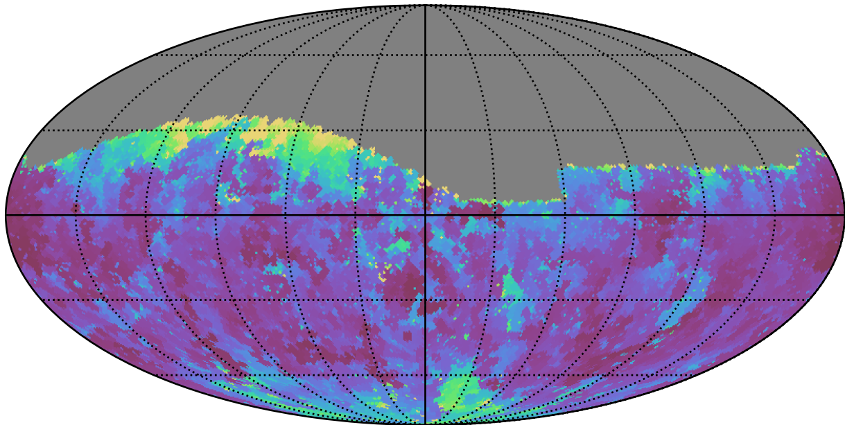
too_100_4v3.4_10yrs Yr 1 g band: Min seeingGeom
