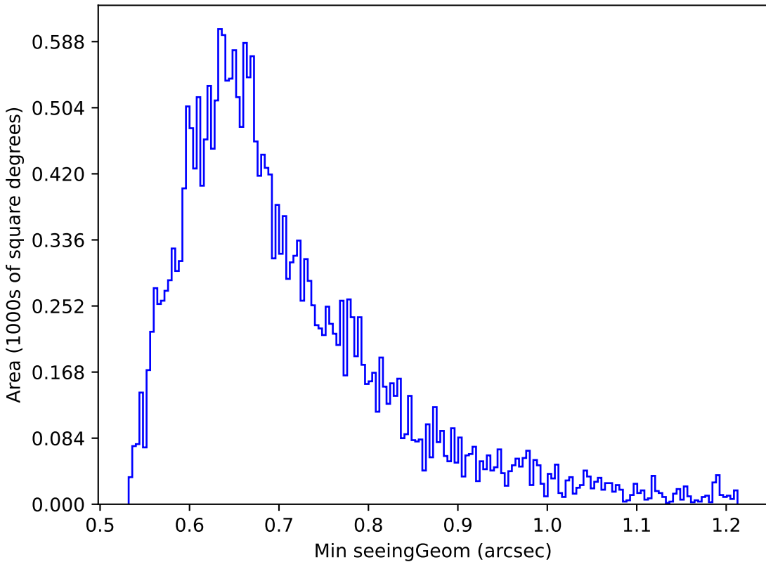
too_100_4v3.4_10yrs Yr 1 g band: Min seeingGeom
