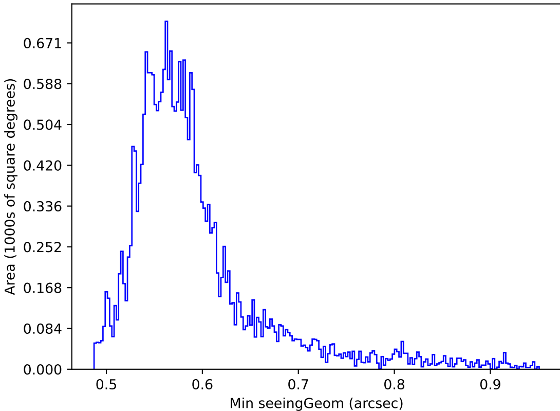
too_100_4v3.4_10yrs Yr 1 all bands: Min seeingGeom
