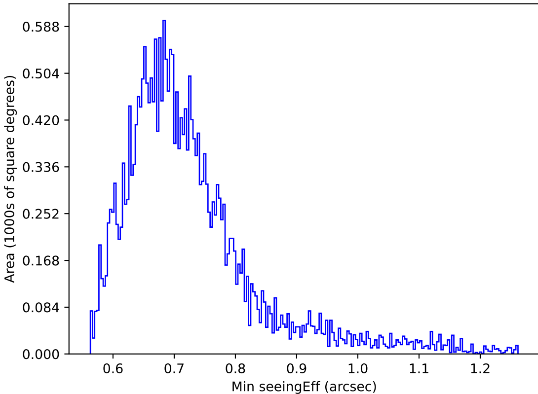
too_100_4v3.4_10yrs Yr 1 z band: Min seeingEff
