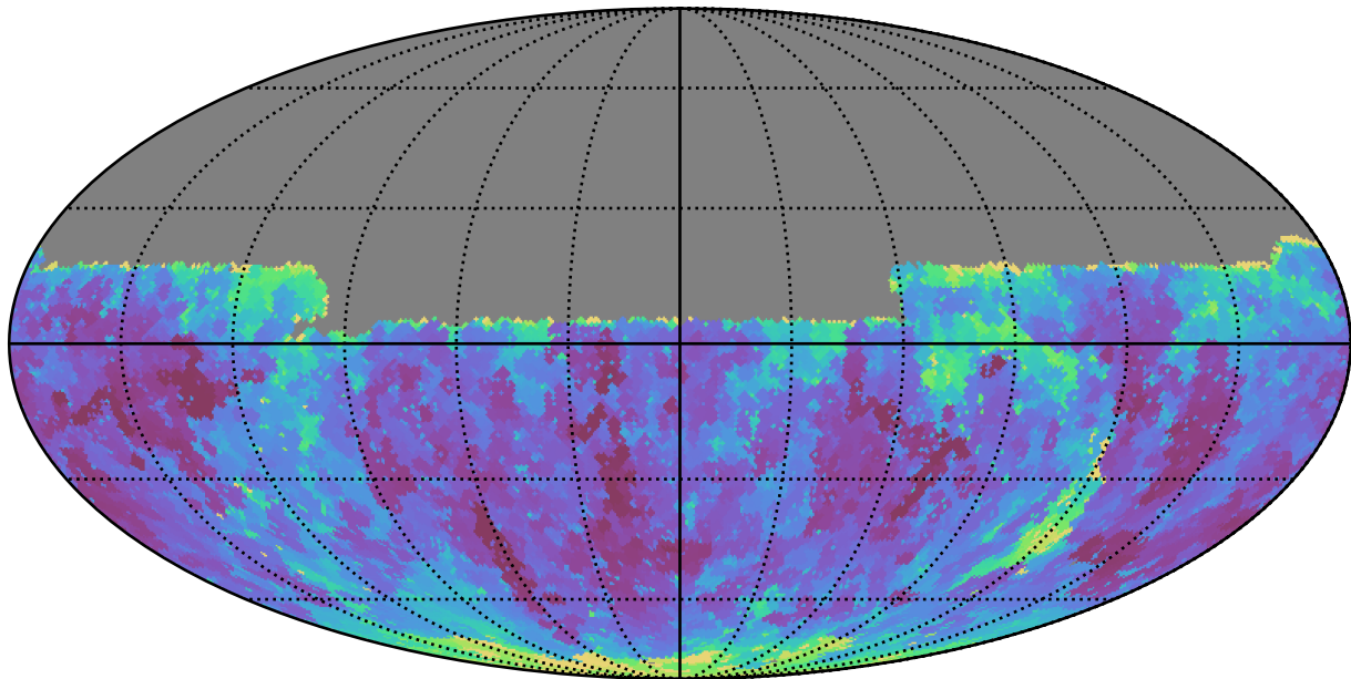
too_100_4v3.4_10yrs Yr 1 y band: Min seeingEff
