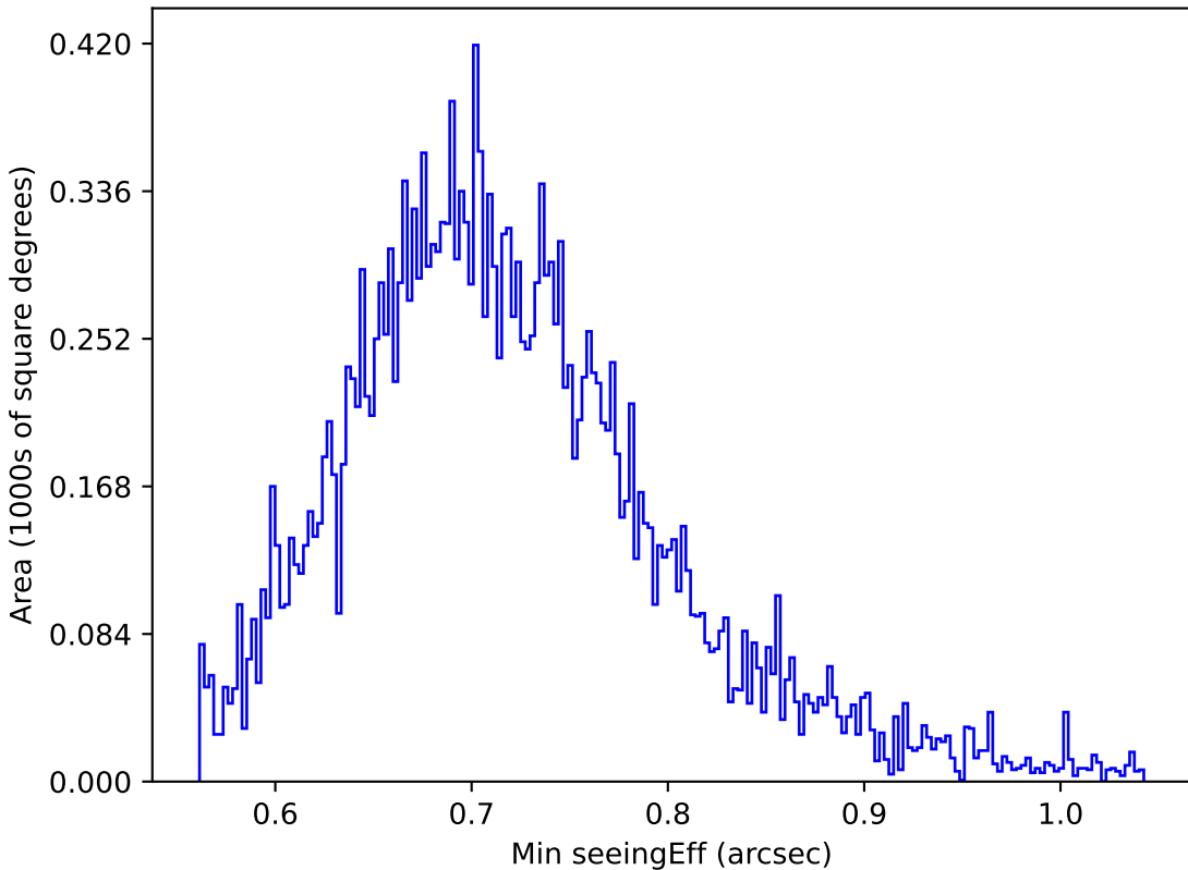
too_100_4v3.4_10yrs Yr 1 y band: Min seeingEff
