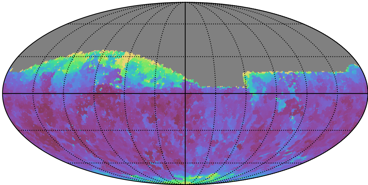
too_100_4v3.4_10yrs Yr1 r band: Min seeingEff
