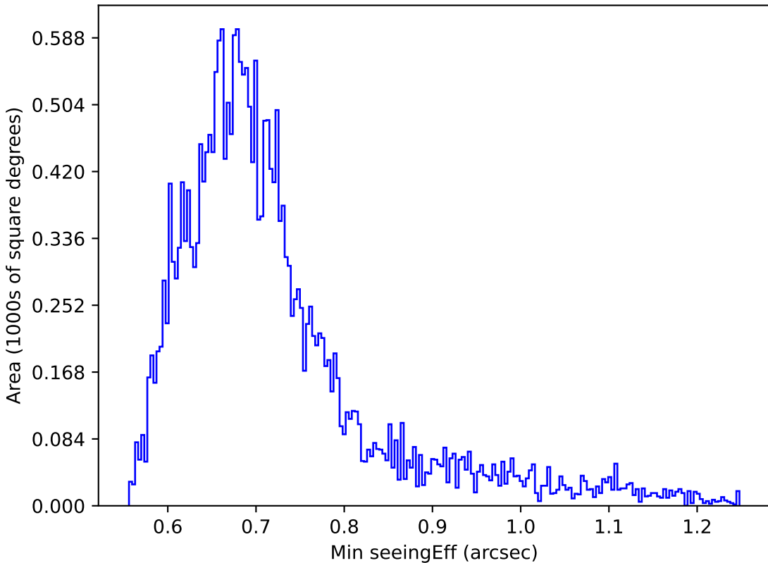
too_100_4v3.4_10yrs Yr 1 r band: Min seeingEff
