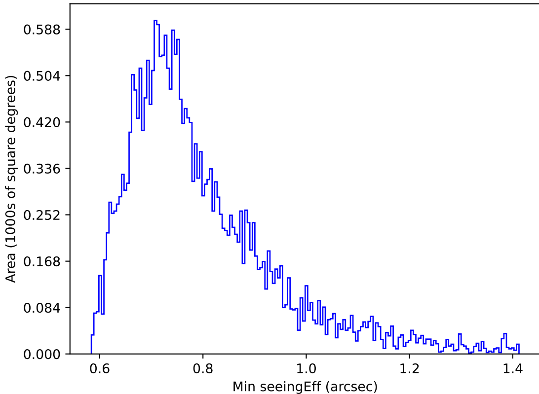
too_100_4v3.4_10yrs Yr 1 g band: Min seeingEff
