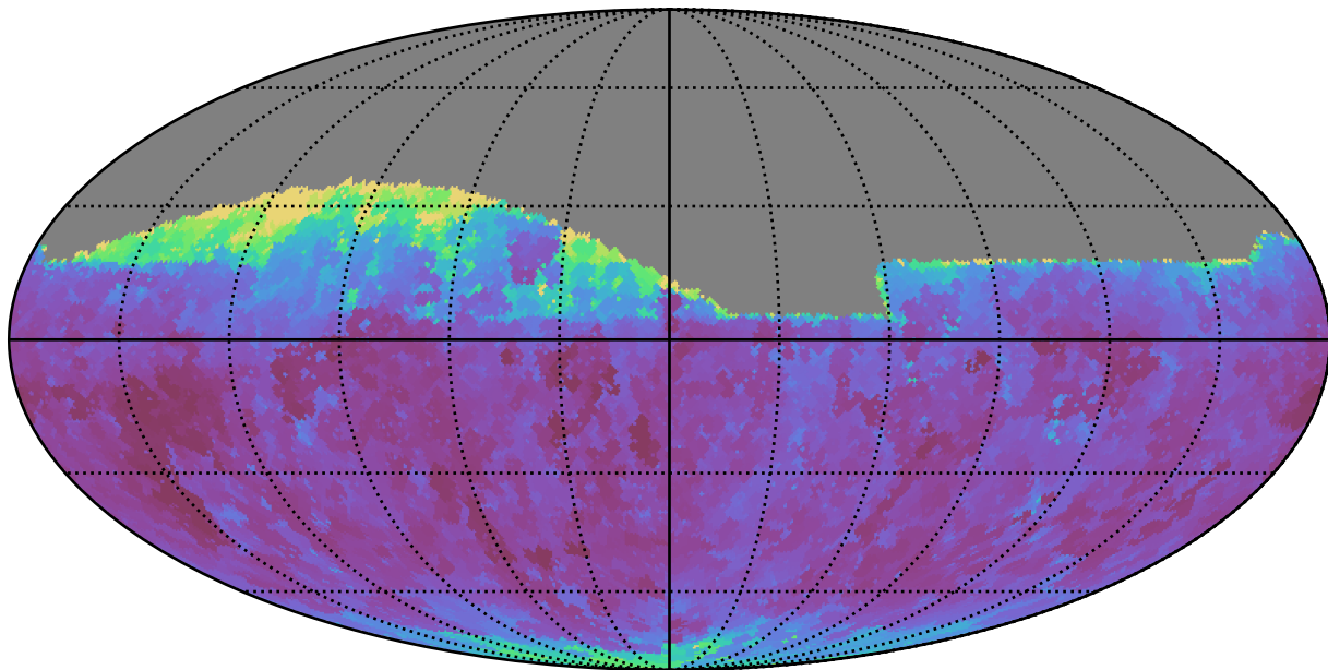
too_100_4v3.4_10yrs Yr 1 all bands: Min seeingEff
