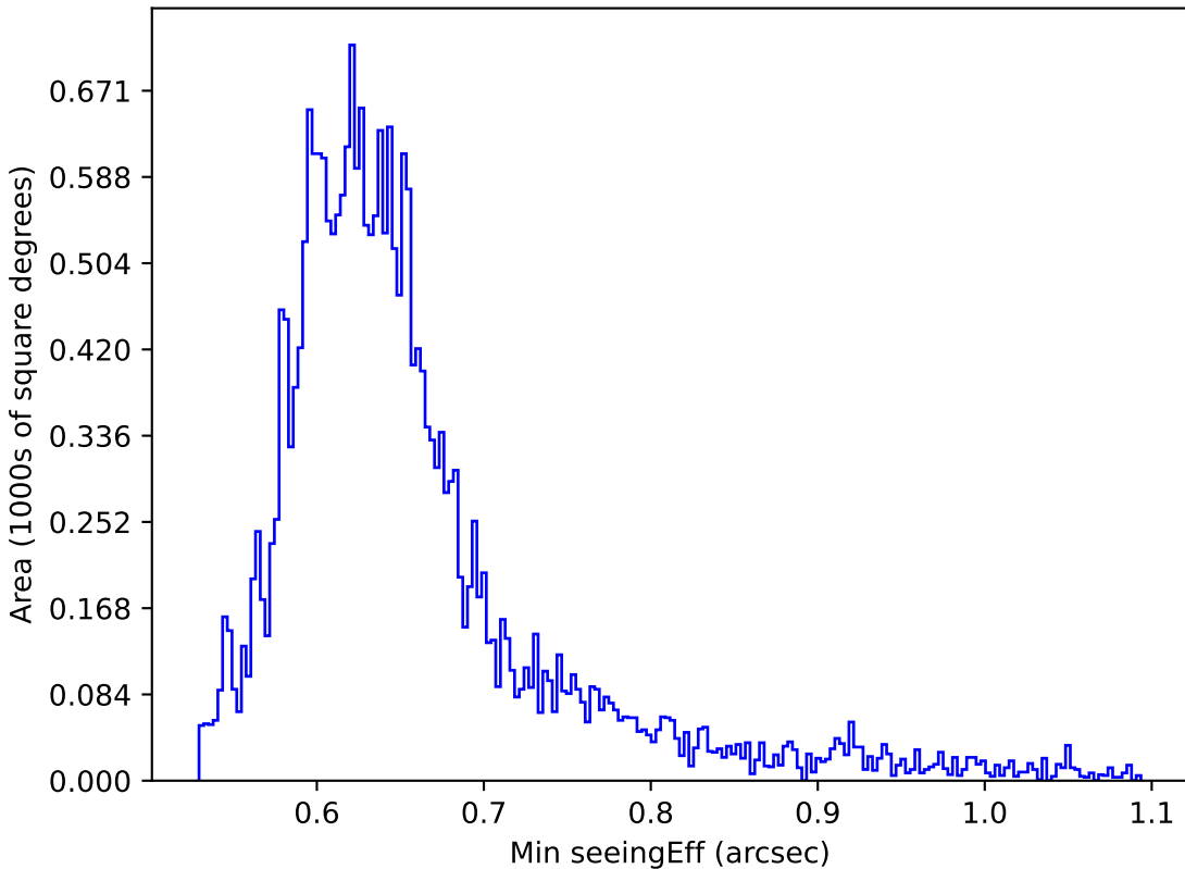
too_100_4v3.4_10yrs Yr 1 all bands: Min seeingEff
