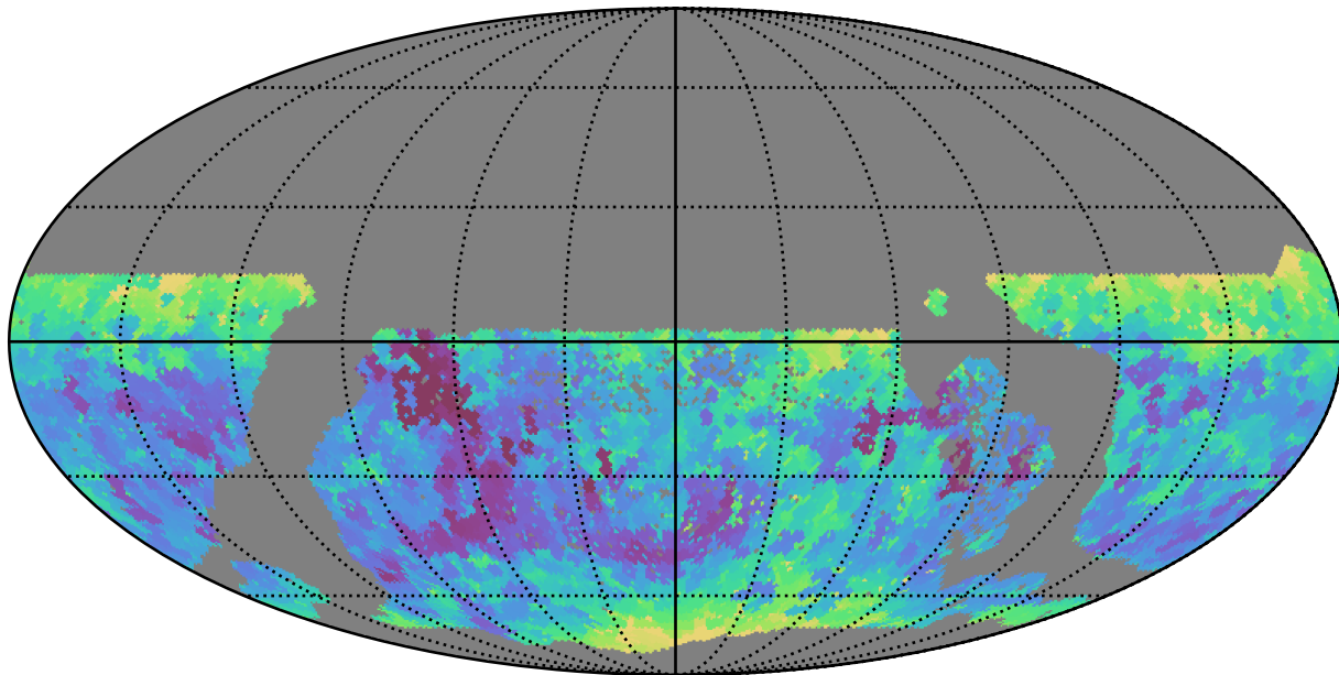
too_100_4v3.4_10yrs WFD z band: Min seeingEff
