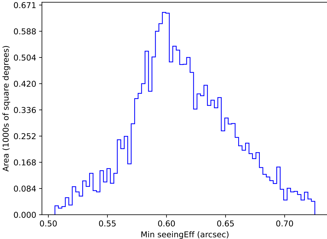
too_100_4v3.4_10yrs WFD z band: Min seeingEff
