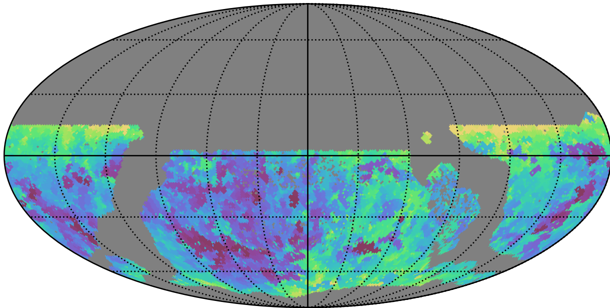
too_100_4v3.4_10yrs WFD r band: Min seeingEff
