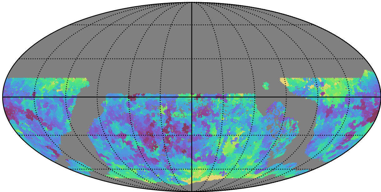
too_100_4v3.4_10yrs WFD g band: Min seeingEff
