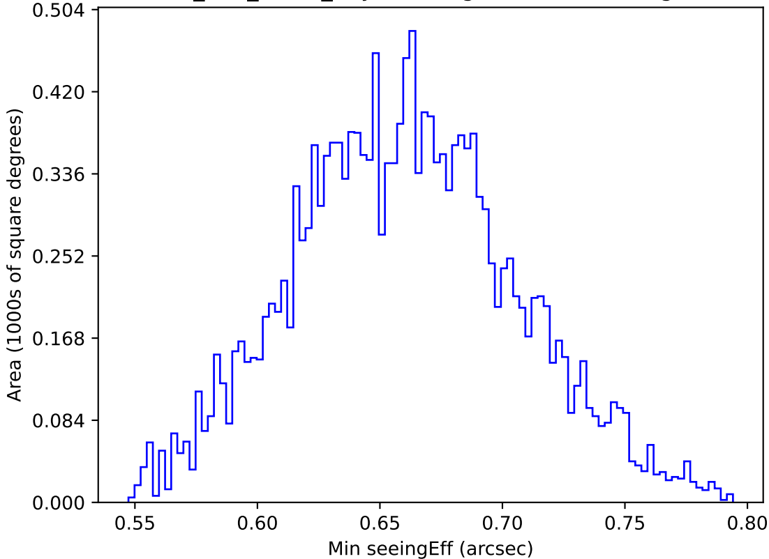
too_100_4v3.4_10yrs WFD g band: Min seeingEff
