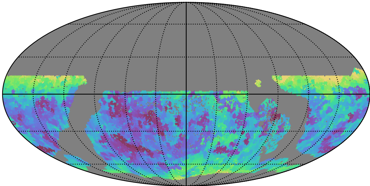
too_100_4v3.4_10yrs WFD all bands: Min seeingEff
