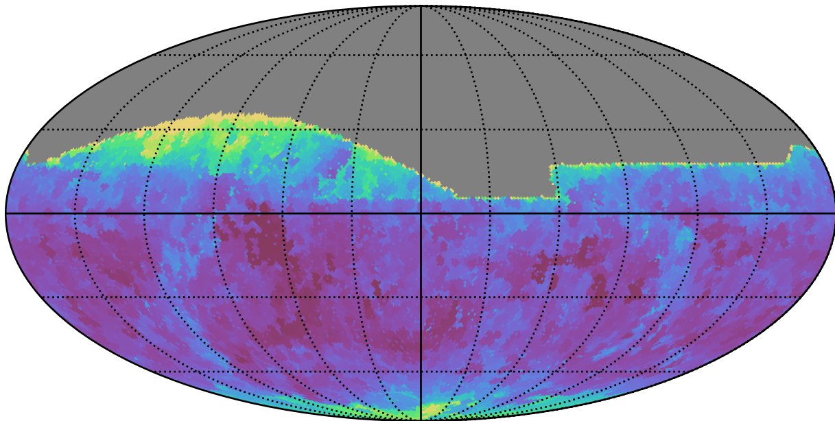
too_100_4v3.4_10yrs All sky z band: Min seeingEff
