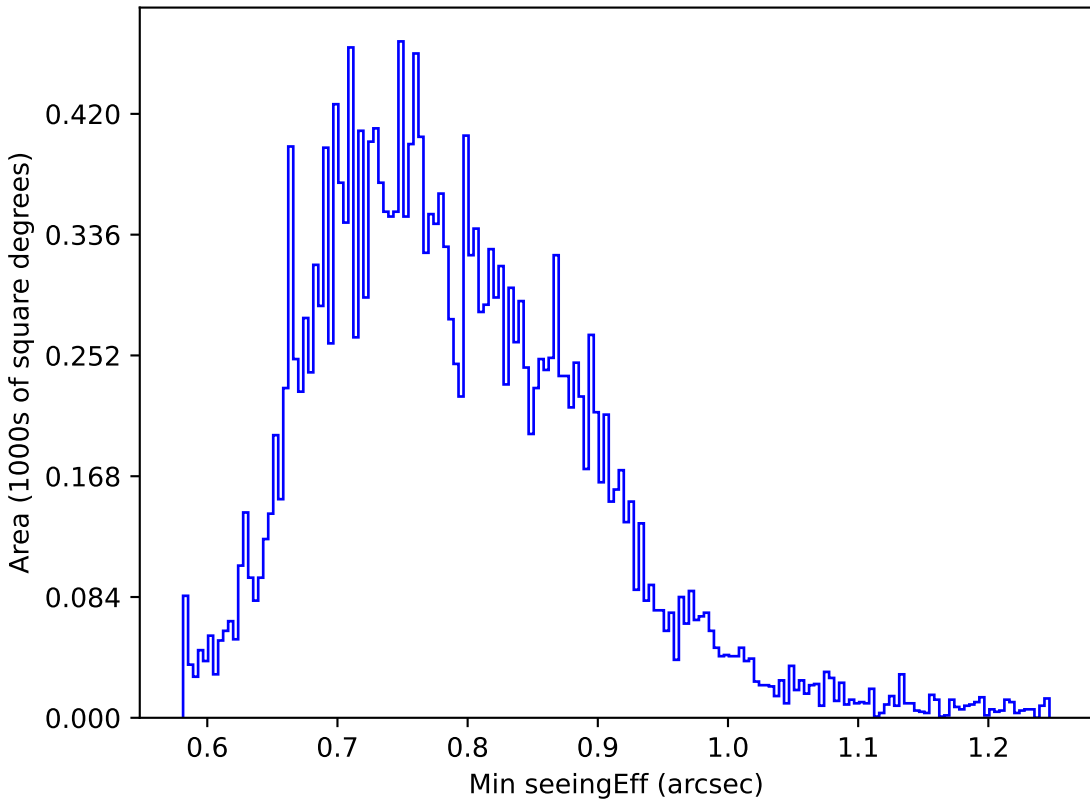
too_100_4v3.4_10yrs All sky u band: Min seeingEff
