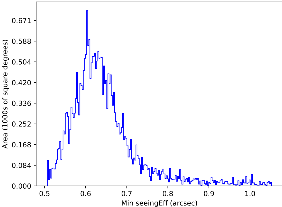
too_100_4v3.4_10yrs All sky r band: Min seeingEff
