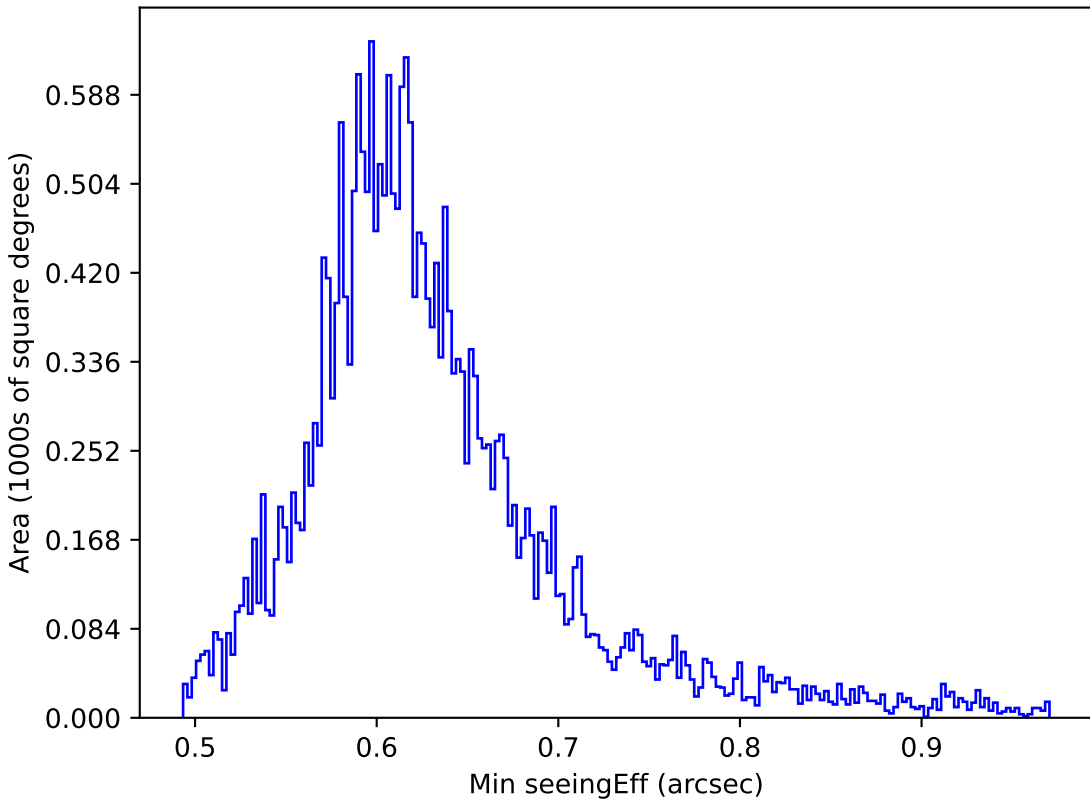
too_100_4v3.4_10yrs All sky i band: Min seeingEff
