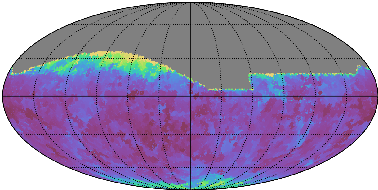
too_100_4v3.4_10yrs All sky g band: Min seeingEff
