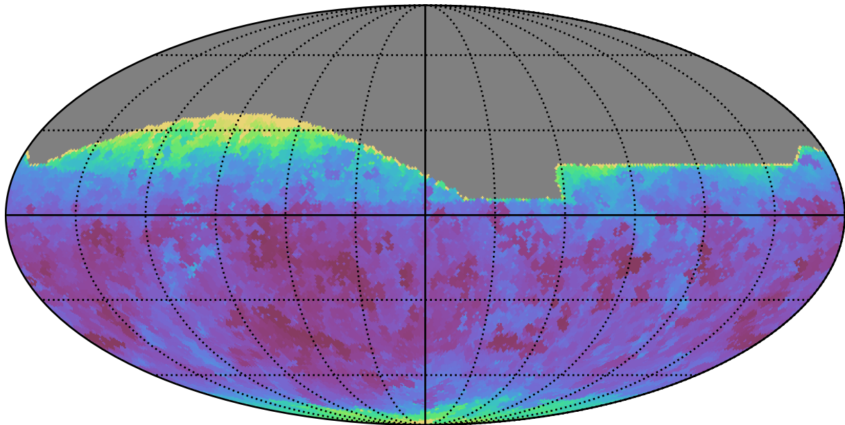
too_100_4v3.4_10yrs All sky all bands: Min seeingEff
