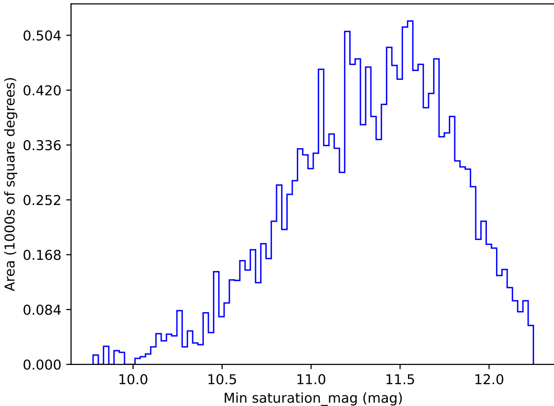
too_100_4v3.4_10yrs WFD u band: Min saturation_mag
