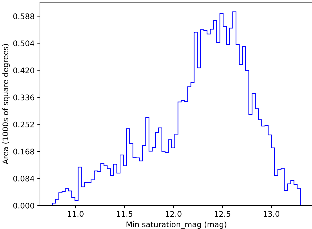
too_100_4v3.4_10yrs WFD i band: Min saturation_mag
