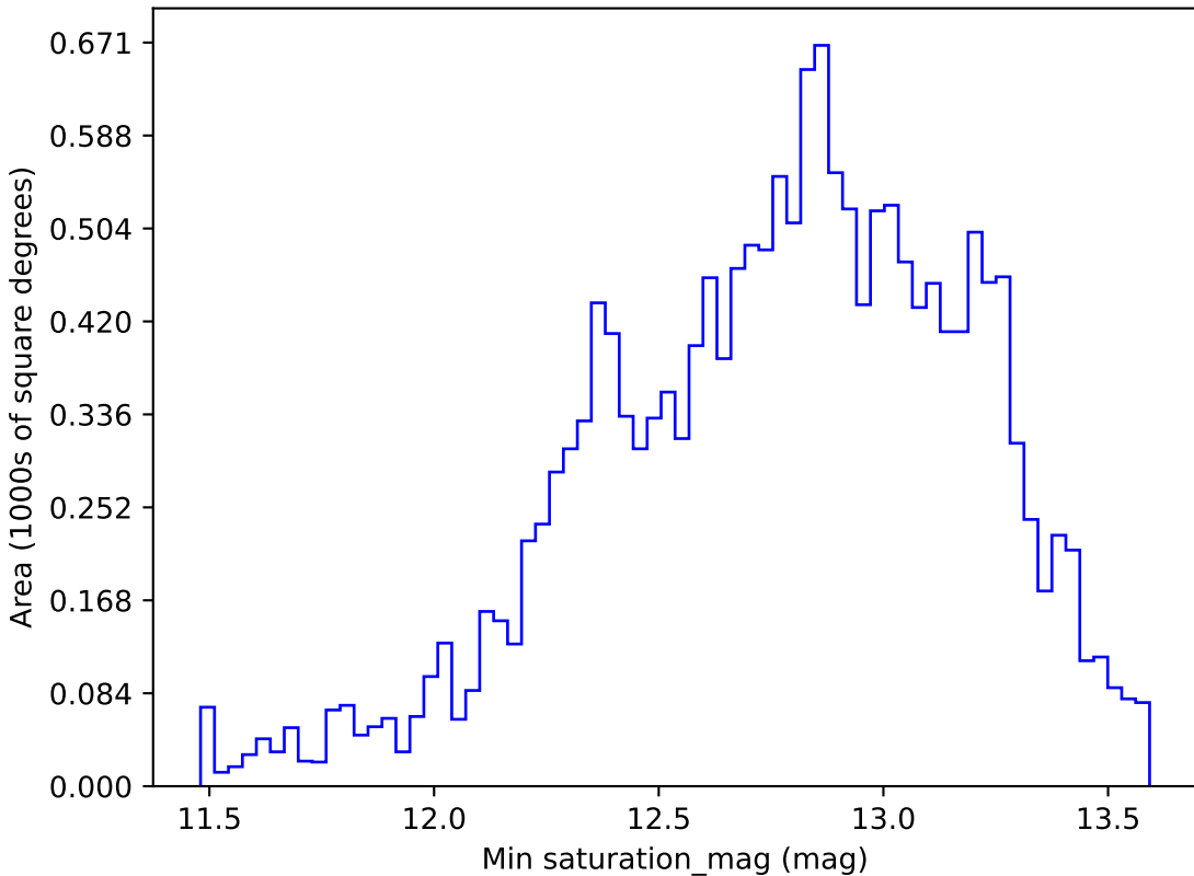
too_100_4v3.4_10yrs WFD g band: Min saturation_mag
