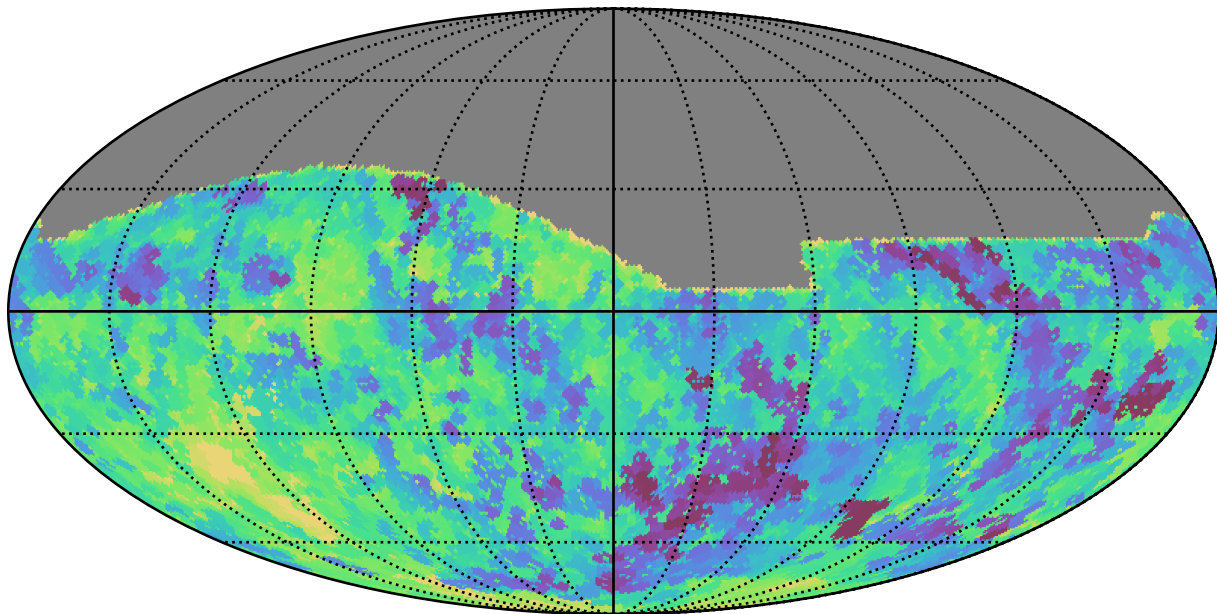
too_100_4v3.4_10yrs All sky z band: Min saturation_mag
