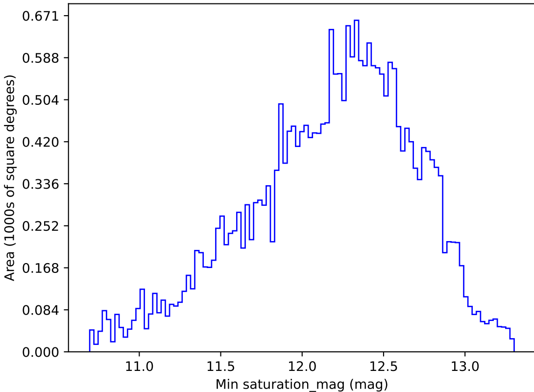
too_100_4v3.4_10yrs All sky z band: Min saturation_mag
