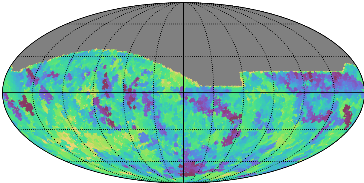
too_100_4v3.4_10yrs All sky i band: Min saturation_mag
