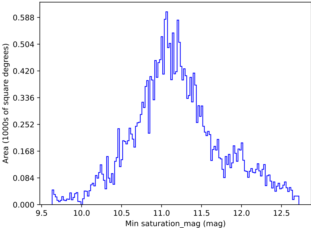
too_100_4v3.4_10yrs All sky all bands: Min saturation_mag
